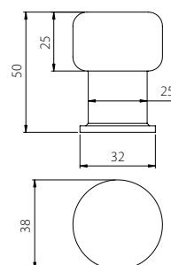
DSS05 Door Stop Stainless Steel Floor Mount or Wall Mount
